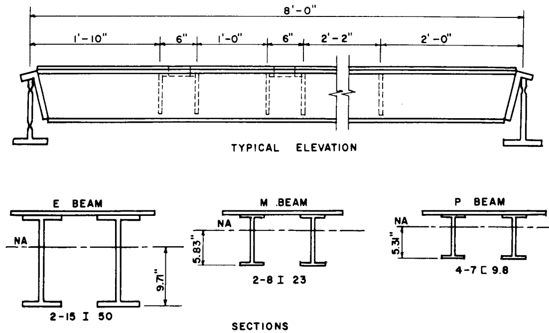
Fig. 4—Elevation and sections of beam strips.
